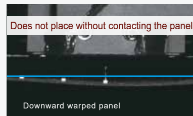
Placement height adjustment
